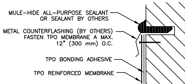
624-A COUNTERFLASHING TERMINATION
