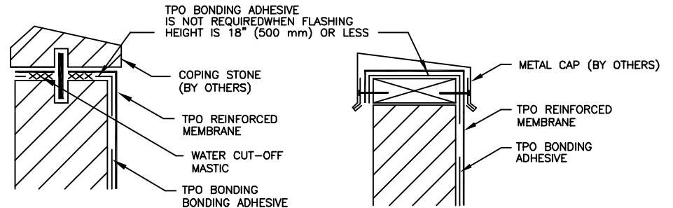
624-D COPING STONE TERMINATION
